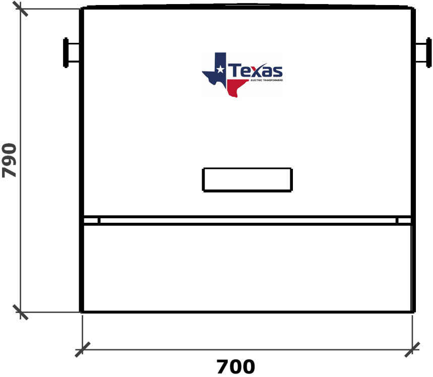
VISTA FRONTAL
